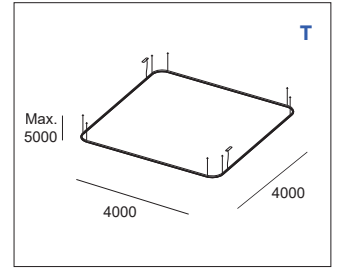
319 W 16973-22085 lm
